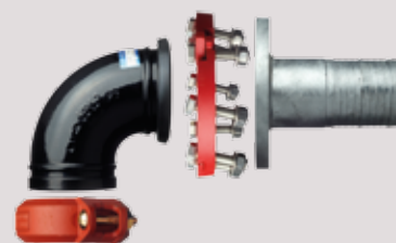
VICTAULIC COUPLING Bravo 400–900 See page 34.
